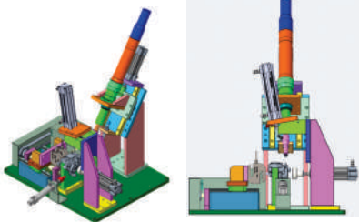
FRONT CALIPER BLEEDER TORQUING & PISTON SLIDING FIXTURE
