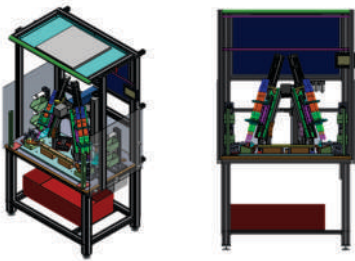
SCREW TORQUING FIXTURE
