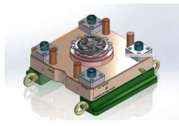
RIVETING MACHINE FOR CLUTCH HOUSING
